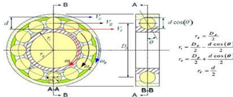
Fig 3. Rolling element bearing geometry
